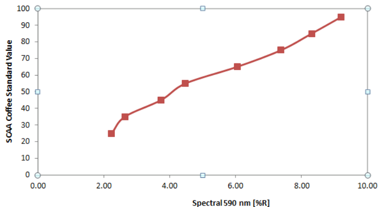
SCAA Coffee Standard Values versus 590 nm Reflectance - multi-segment fit
